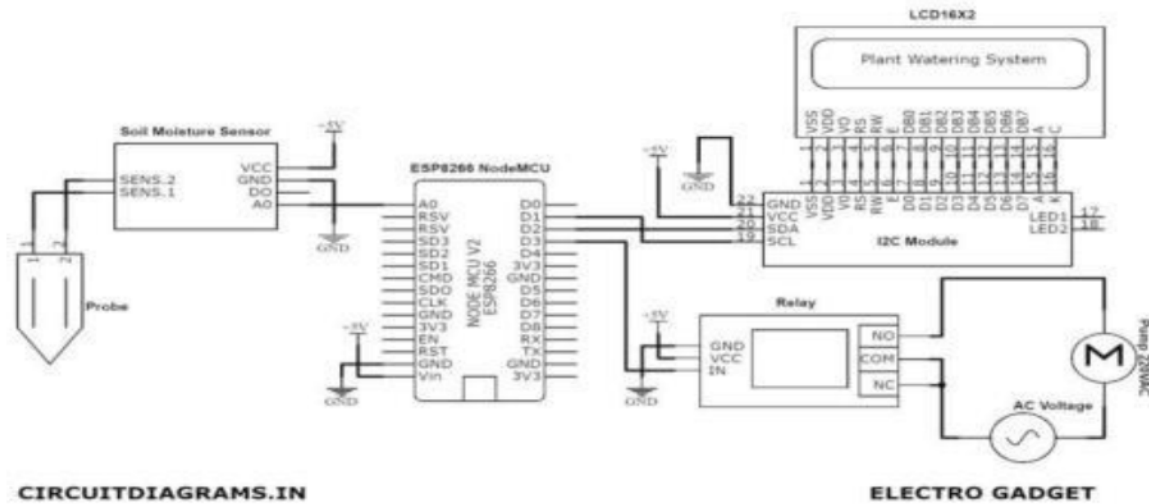
Fig 1: Circuit Diagram of smart plant watering system
