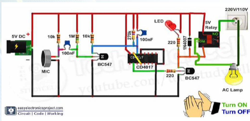
Fig 1: Circuit Diagram of Automatic home control system using sound Technology
